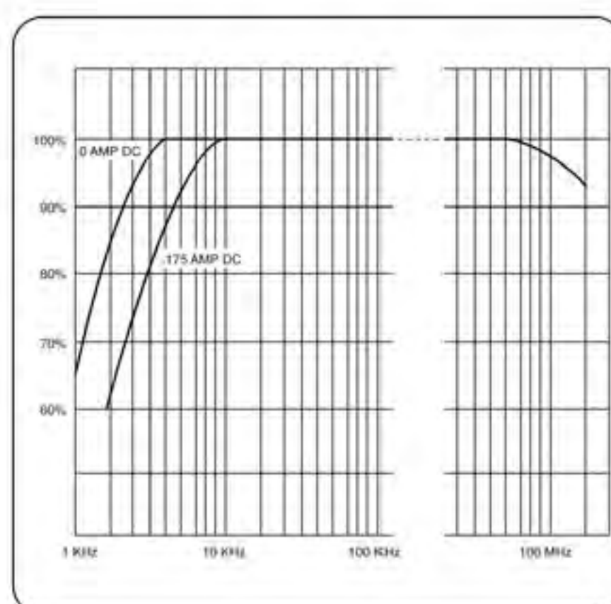
► CT2 Typical Frequency Response.
