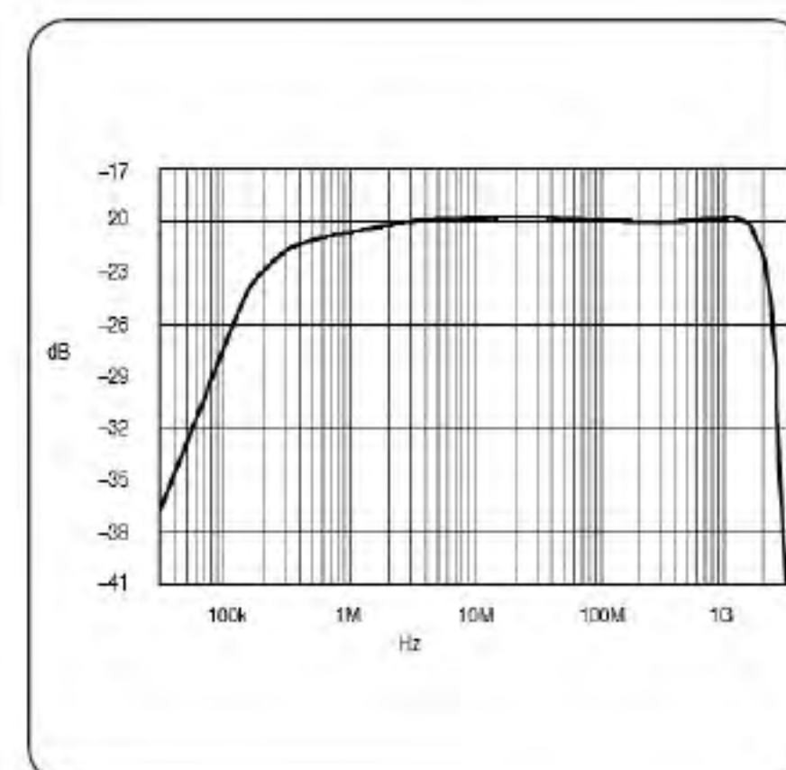
► CT6 Typical Frequency Response.
