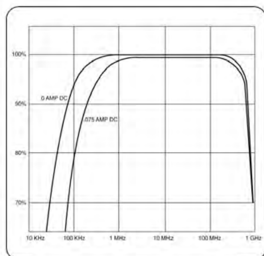
► CT1 Typical Frequency Response.
